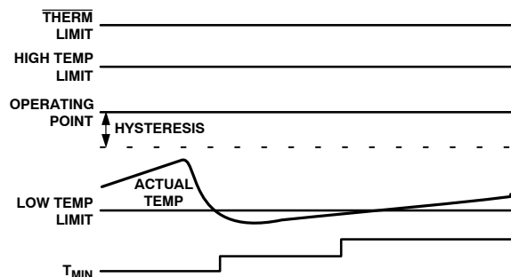
Figure 72. Increasing T_{MIN} for Quieter Operation
