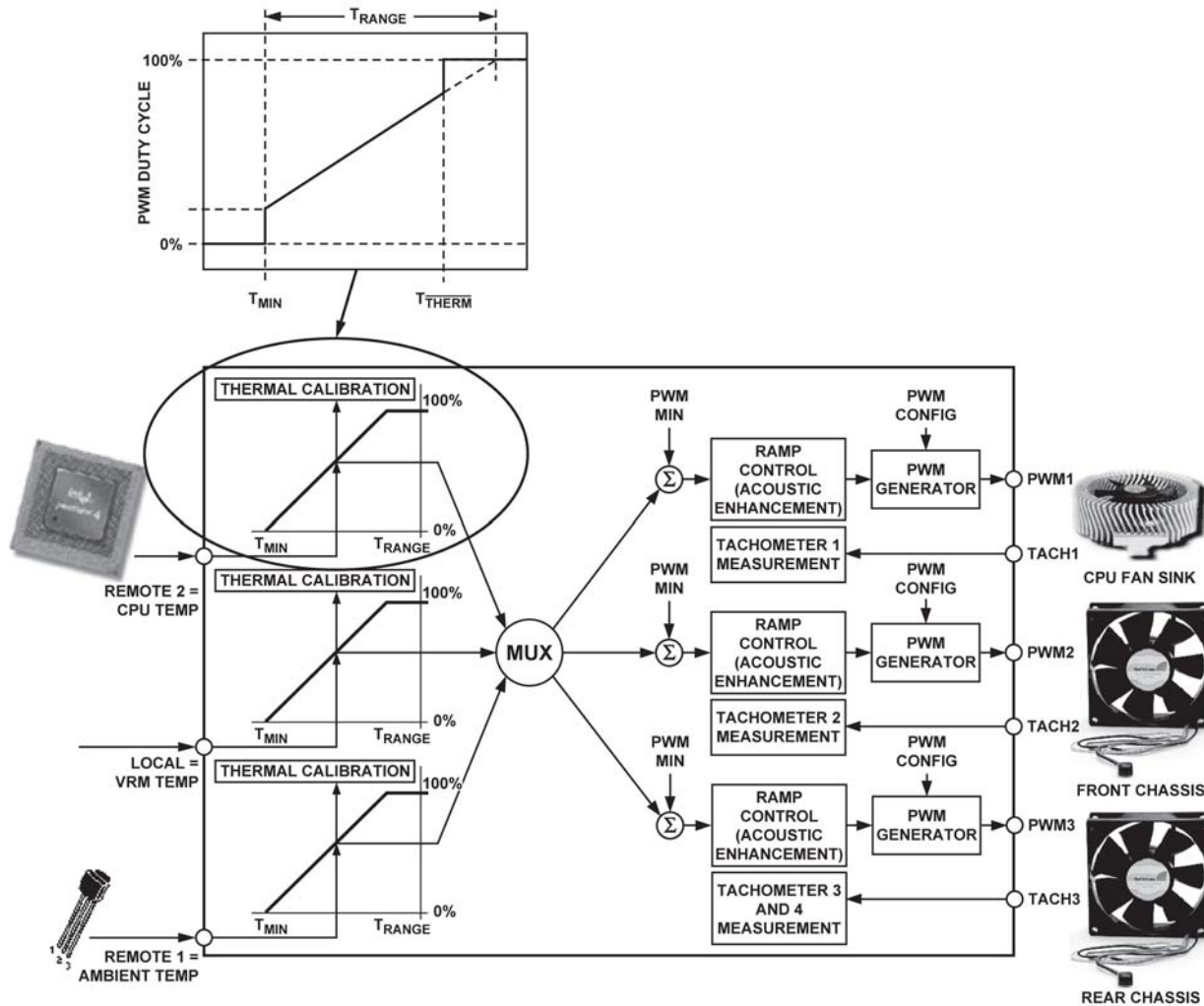
Figure 62. How T_{THERM} Relates to Automatic Fan Control
