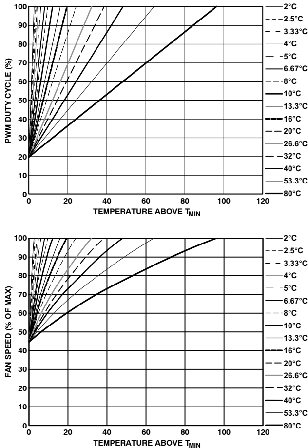
Figure 60. T_{\text{RANGE}} and % Fan Speed Slopes with \text{PWM}_{\text{MIN}} = 20\%
