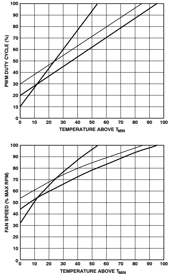
Figure 61. T_{\text{RANGE}} and % Fan Speed Slopes for VRM, Ambient, and CPU Temperature Channels
