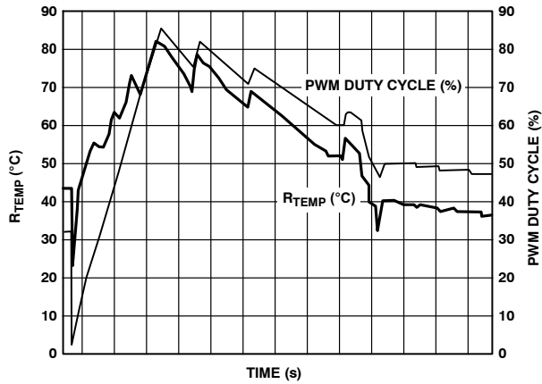
Figure 81. How Fan Reacts to Temperature Variation in Enhanced Acoustics Mode
