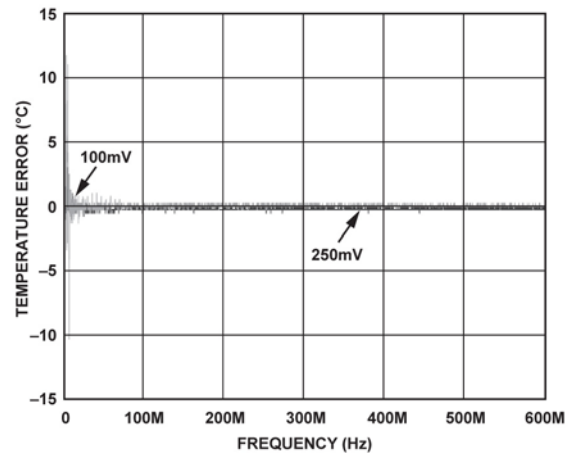
Figure 8. Internal Temperature Error vs. Frequency
