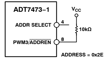
Figure 13. Default SMBus Address = 0x2E
