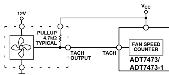
Figure 40. Fan with TACH Pullup to V_{CC}
