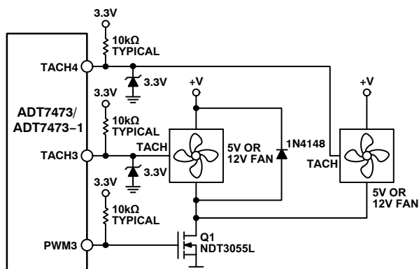
Figure 39. Interfacing Two Fans in Parallel to the PWM3 Output Using a Single N-Channel MOSFET
