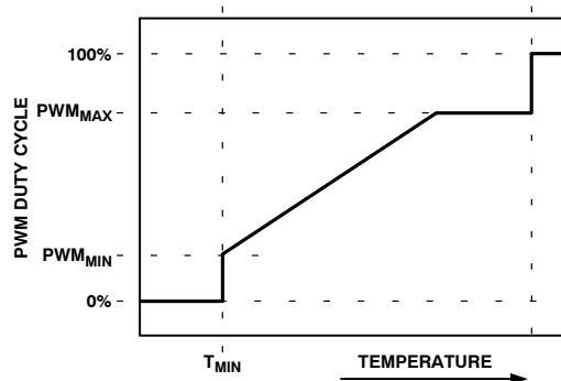
Figure 55. PWM MAX Determines Maximum PWM Duty Cycle Below the THERM Temperature Limit
