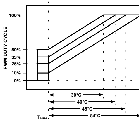
Figure 58. Increasing PWM MIN Changes Effective T RANGE
