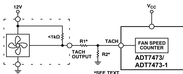
Figure 43. Fan with Strong TACH pullup to > V CC or Totem-Pole Output, Attenuated with R1/R2
