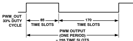
Figure 75. 33% PWM Duty Cycle Represented in Time Slots
