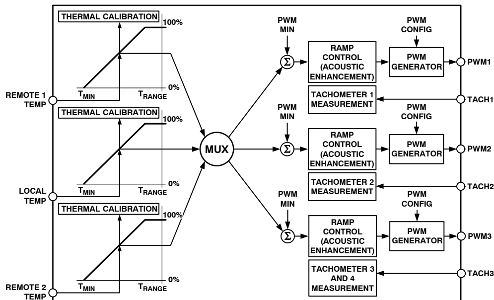
Figure 47. Automatic Fan Control Block Diagram
