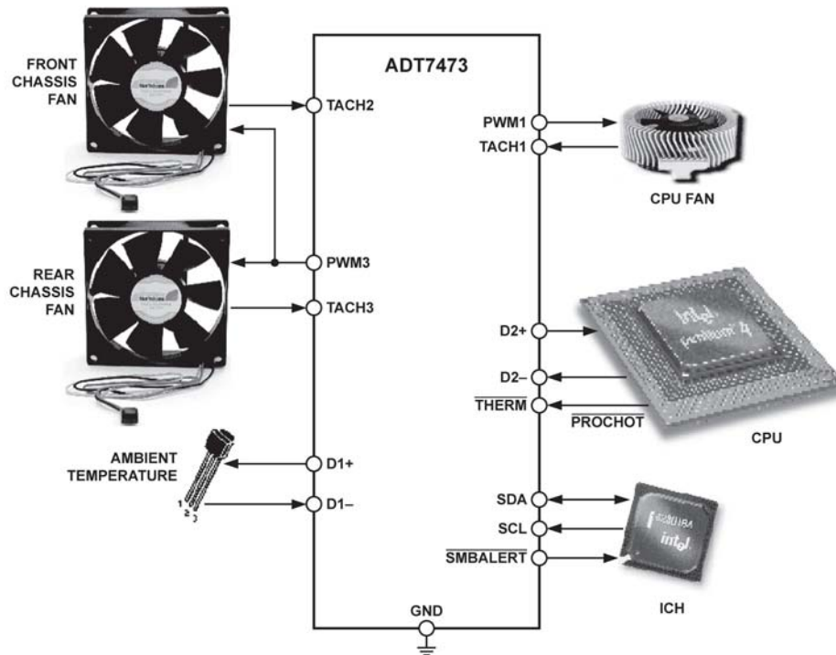
Figure 49. Recommended Implementation 1
