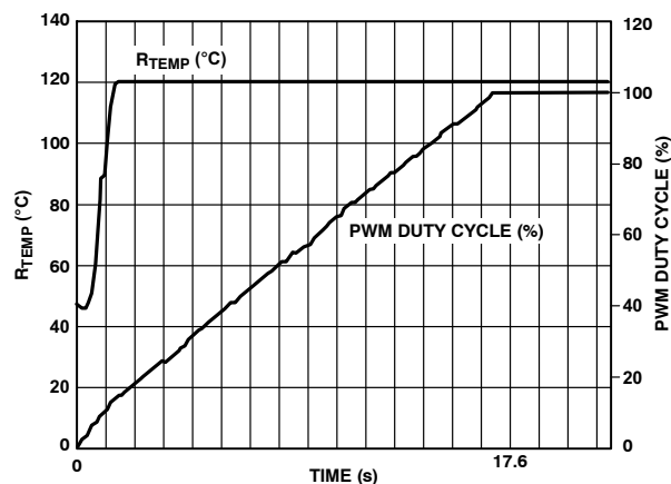
Figure 79. Enhanced Acoustics Mode with Ramp Rate = 2
