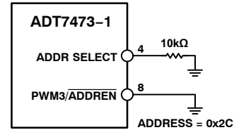
Figure 14. SMBus Address = 0x2C (Pin4 = 0)
