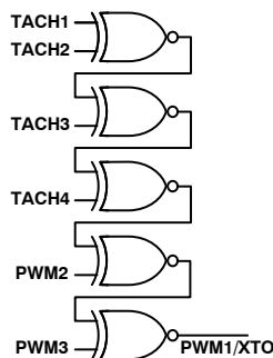
Figure 45. XNOR Tree Test
