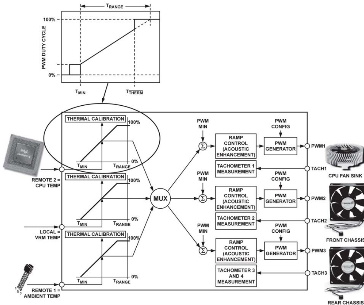
Figure 63. The T_{HYST} Value Applies to Fan On/Off Hysteresis and T_{THERM} Hysteresis
