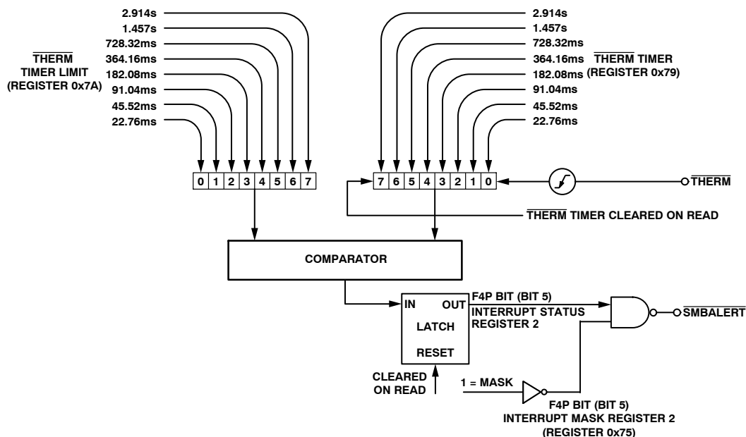
Figure 33. Functional Block Diagram of the ADT7473 THERM Monitoring Circuitry
