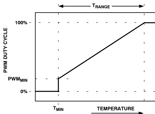
Figure 56. T RANGE Parameter Affects Cooling Slope
