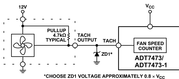
Figure 41. Fan with TACH Pullup to Voltage > 3.6 V Clamped with Zener Diode
