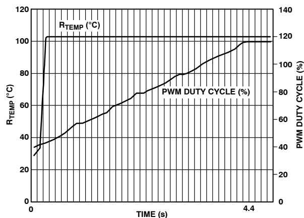
Figure 78. Enhanced Acoustics Mode with Ramp Rate = 8
