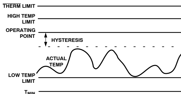
Figure 70. Temperature Between Operating Point and Low Temperature Limit
