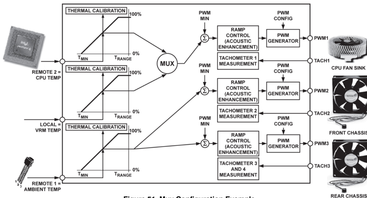
Figure 51. Mux Configuration Example
