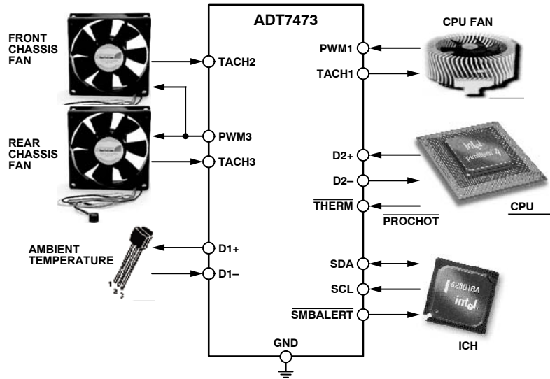
Figure 12. ADT7473 Configuration
