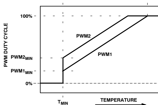
Figure 54. Operating Two Different Fans from a Single Temperature Channel
