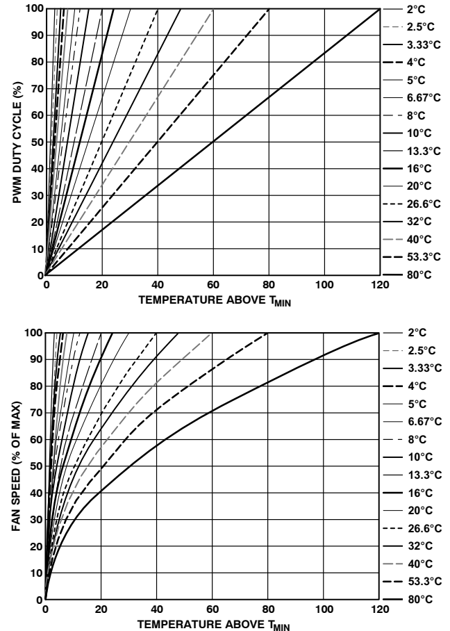
Figure 59. T_{RANGE} vs. Actual Fan Speed Profile
