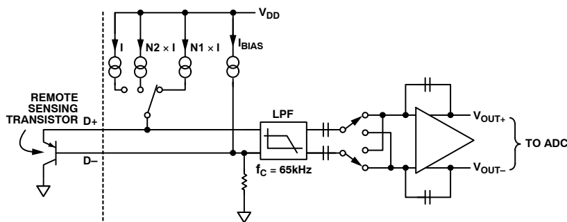
Figure 24. Signal Conditioning for Remote Diode Temperature Sensors
