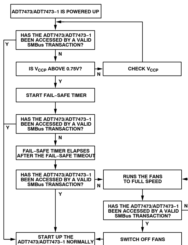
Figure 46. Power-On Flow Chart
