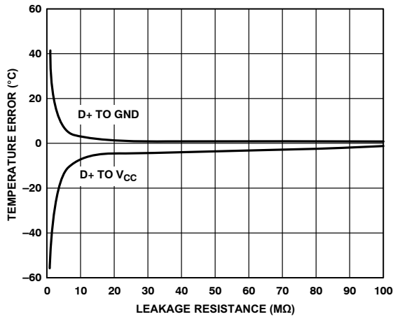
Figure 3. Remote Temperature Error vs. PCB Resistance
