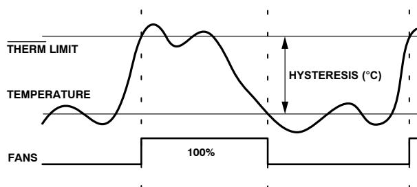
Figure 28. THERM Limit Operation
