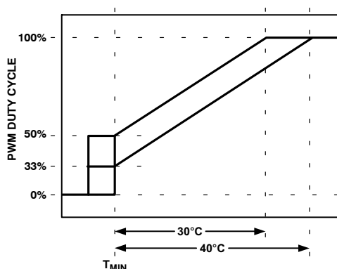
Figure 57. Adjusting PWM MIN Affects T RANGE
