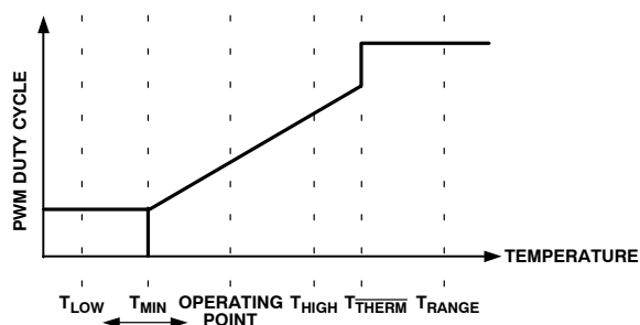
Figure 66. Dynamic T_{MIN} Control Loop
