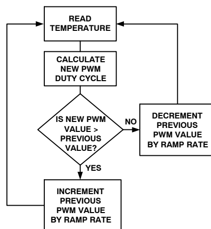
Figure 76. Enhanced Acoustics Algorithm
