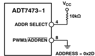
Figure 15. SMBus Address = 0x2D (Pin 4 = 1)
