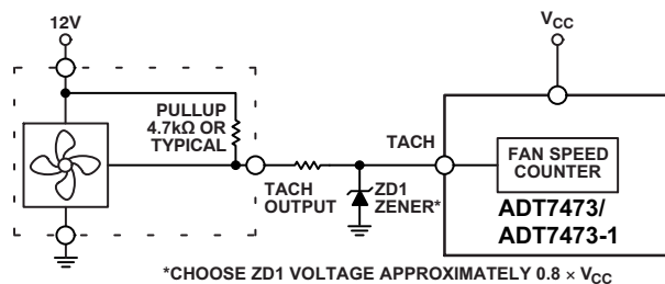
Figure 42. Fan with Strong TACH Pullup to > V_{CC} or Totem-Pole Output, Clamped with Zener and Resistor
