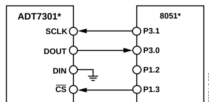
Figure 16. ADT7301-to-8051 Interface
