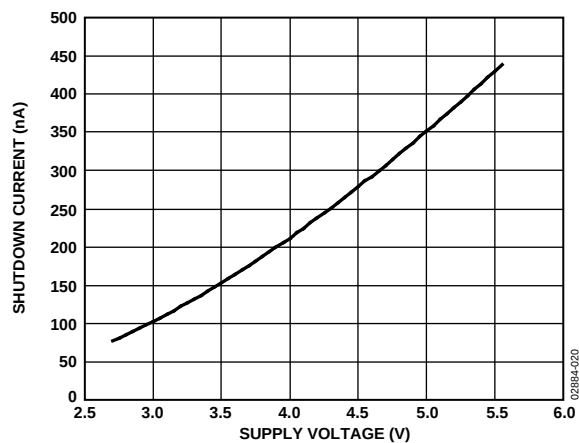
Figure 8. Shutdown Current vs. Supply Voltage @ 30^{\circ}C
