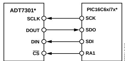
Figure 17. ADT7301-to-PIC16C6x/7x Interface
