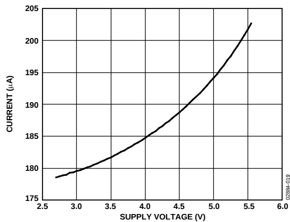
Figure 7. Average Operating Supply Current vs. Supply Voltage @ 30^{\circ}C
