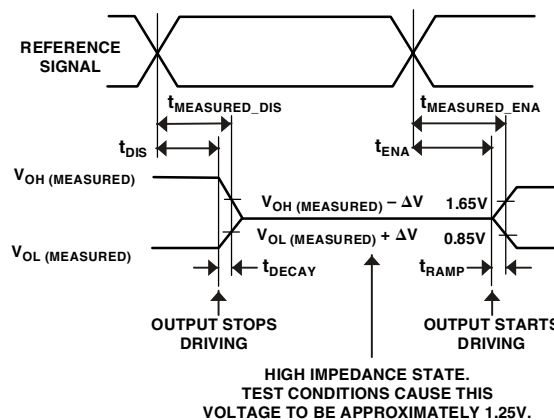
Figure 35. Output Enable/Disable
