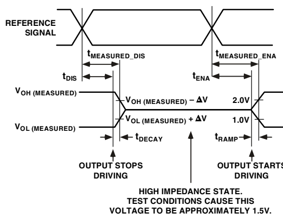
Figure 23. Output Enable/Disable
