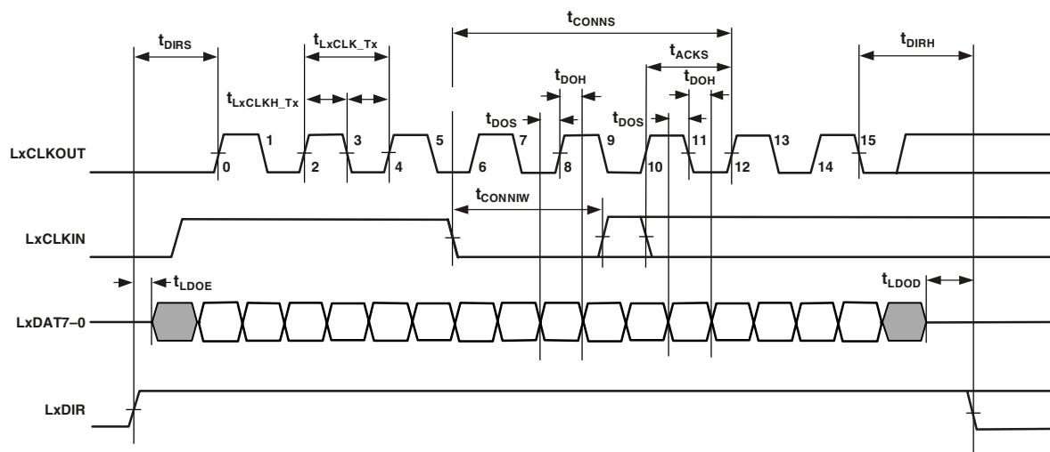
Figure 10. Link Ports—Transmit
