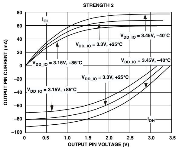
Figure 23. Typical Drive Currents at Strength 2
