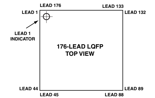
Figure 90. 176-Lead LQFP Lead Configuration (Top View)
