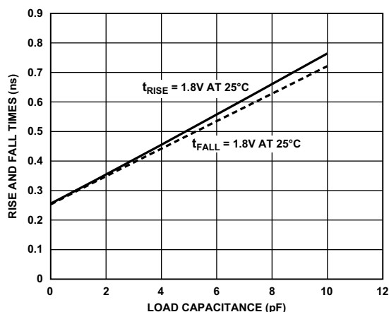
Figure 87. Driver Type B and Driver Type C Typical Rise and Fall Times (10% to 90%) vs. Load Capacitance ( V_{DD\_DMC} = 1.8\text{ V} ) for DDR2
