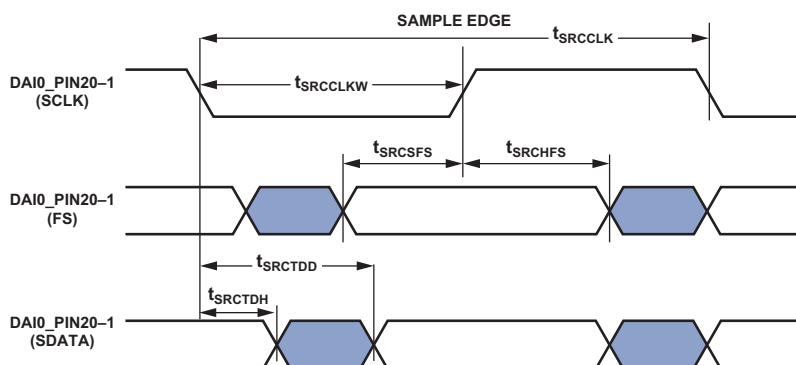
Figure 35. ASRC Serial Output Port Timing
