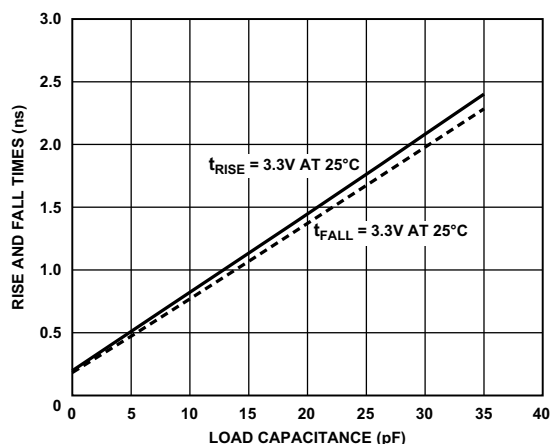
Figure 85. Driver Type H Typical Rise and Fall Times (10% to 90%) vs. Load Capacitance ( V_{DD\_EXT} = 3.3\text{ V} )
