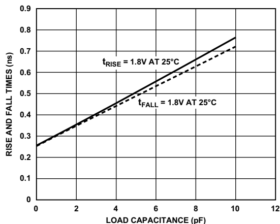
Figure 86. Driver Type B and Driver Type C Typical Rise and Fall Times (10% to 90%) vs. Load Capacitance ( V_{DD\_DMC} = 1.8\text{ V} ) for LPDDR
