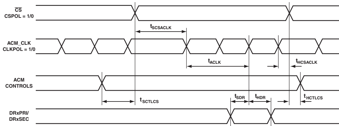
Figure 48. ACM Timing
