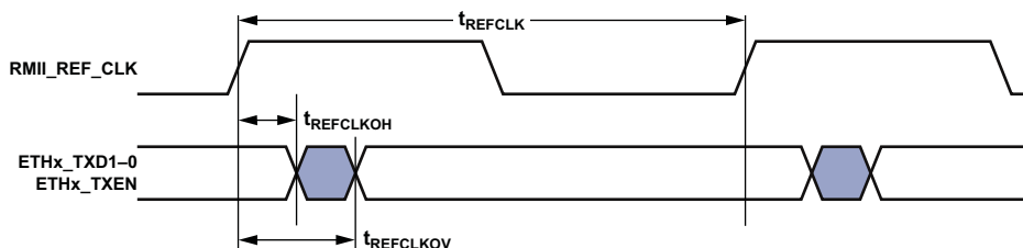
Figure 51. 10/100 Ethernet MAC Controller Timing: RMII Transmit Signal
