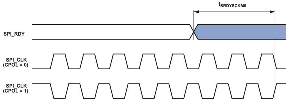
Figure 41. SPI_RDY Setup Before SPI_CLK with CPHA = 0
