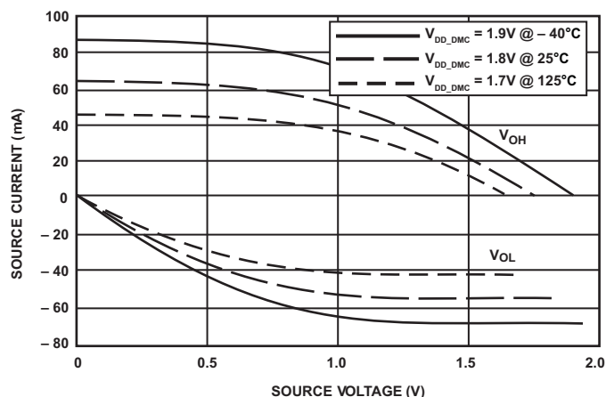
Figure 56. Driver Type B Current ( 1.8\text{ V } V_{DD\_DMC} )
