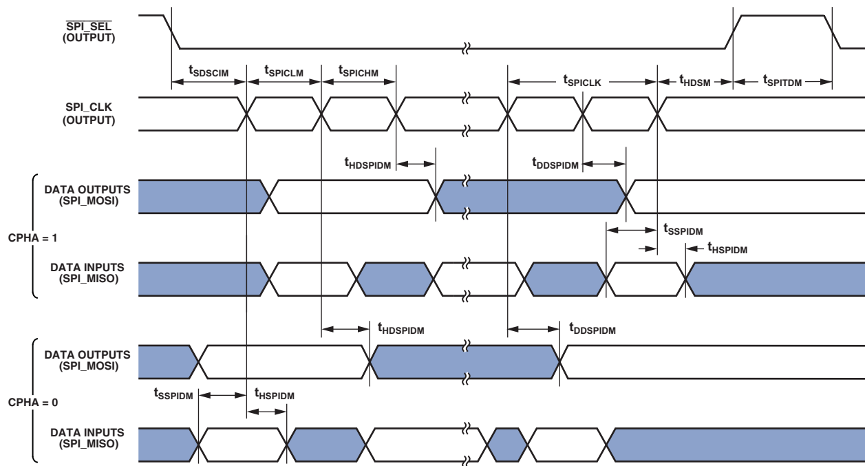
Figure 35. Serial Peripheral Interface (SPI) Port—Master Timing
