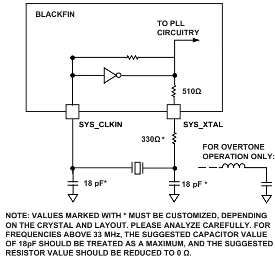
Figure 6. External Crystal Connection
