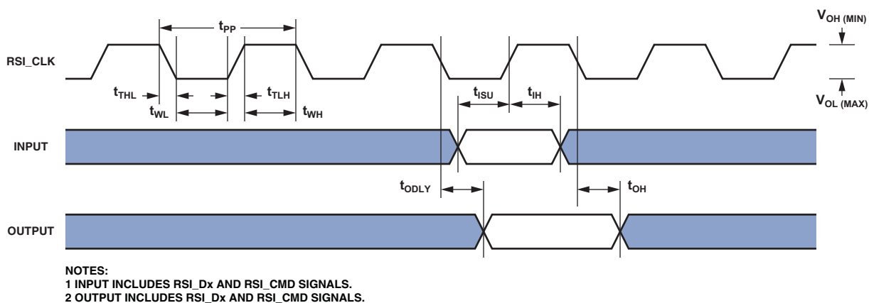
Figure 49. RSI Controller Timing
