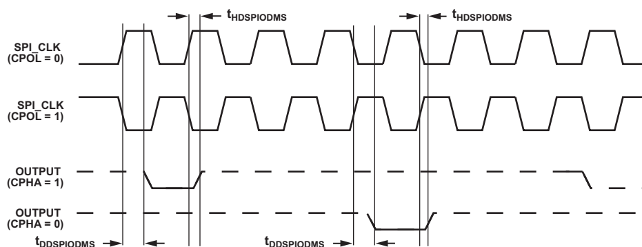
Figure 40. ODM Slave
