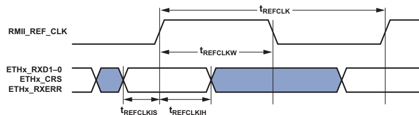
Figure 50. 10/100 Ethernet MAC Controller Timing: RMII Receive Signal
