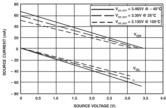
Figure 55. Driver Type A Current ( 3.3\text{ V } V_{DD\_EXT} )
