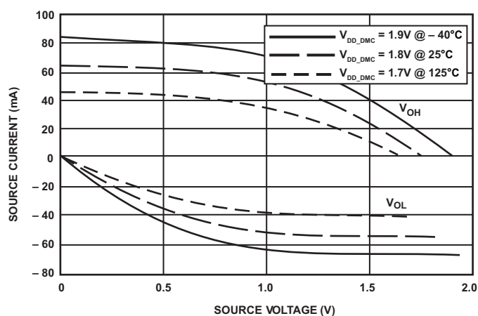
Figure 57. Driver Type C Current ( 1.8\text{ V } V_{DD\_DMC} )
