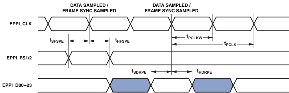
Figure 27. PPI GP Receive Mode with External Frame Sync Timing
