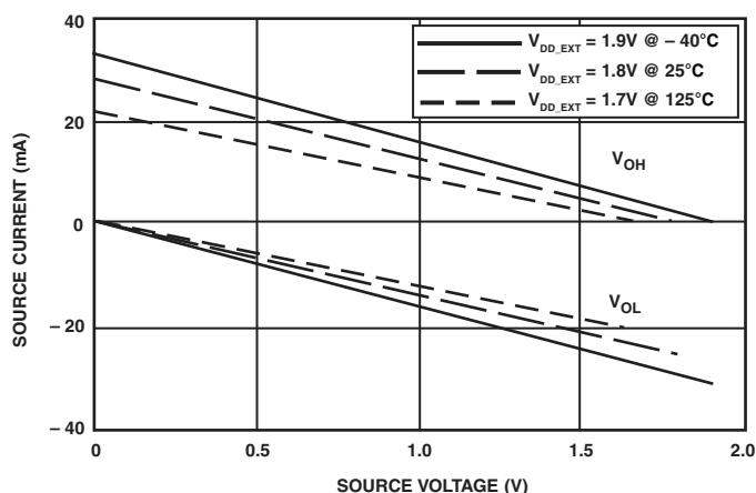
Figure 54. Driver Type A Current ( 1.8\text{ V } V_{DD\_EXT} )
