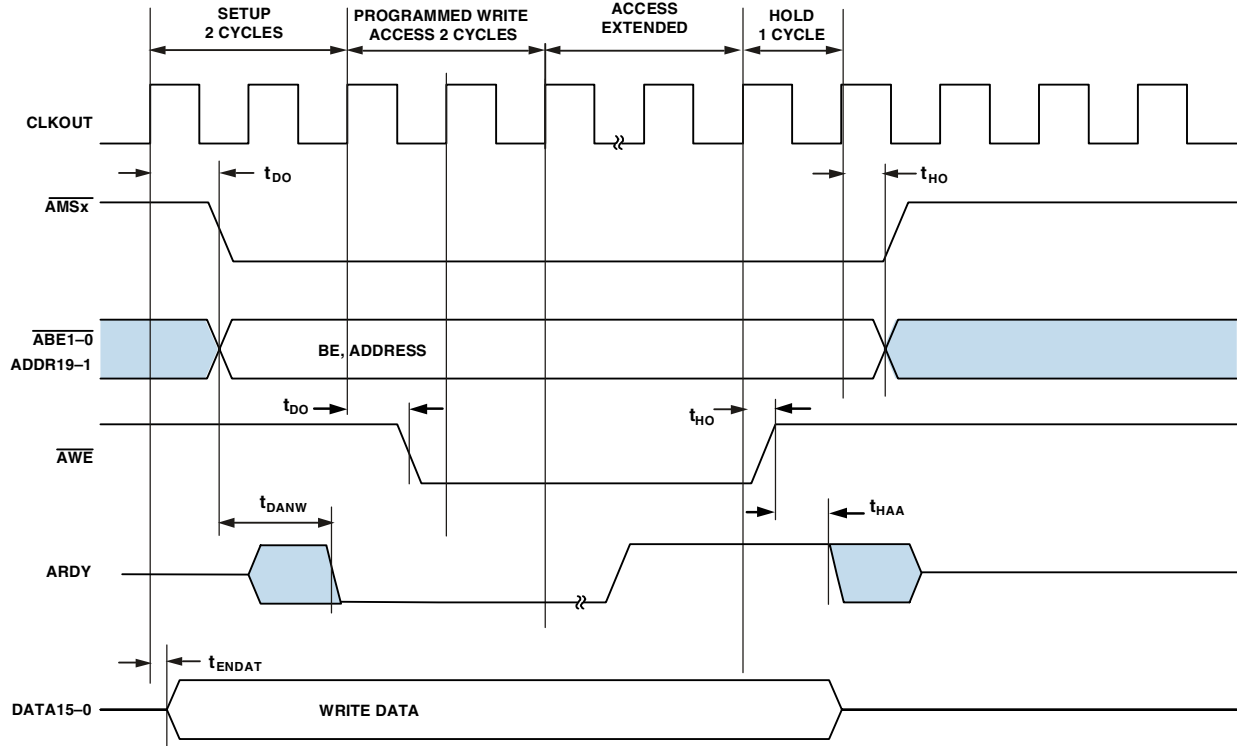
Figure 15. Asynchronous Memory Write Cycle Timing with Asynchronous \overline{\text{ARDY}}
