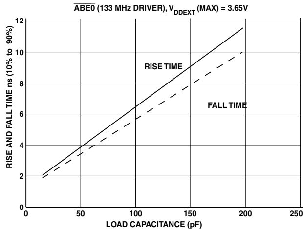
Figure 46. Typical Rise and Fall Times (10%–90%) versus Load Capacitance for Driver A at V_{DDEXT} (max)
