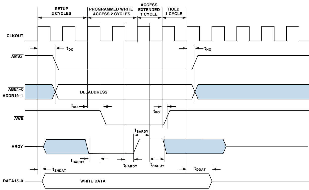
Figure 14. Asynchronous Memory Write Cycle Timing with Synchronous \overline{\text{ARDY}}
