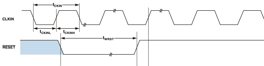
Figure 11. Clock and Reset Timing
