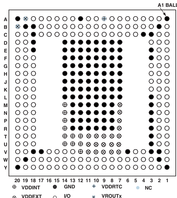
Figure 56. 316-Ball Mini-BGA Pin Configuration (Bottom View)
