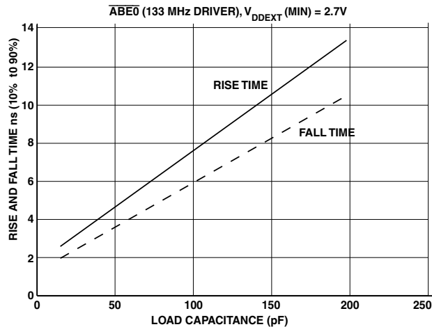
Figure 45. Typical Rise and Fall Times (10%–90%) versus Load Capacitance for Driver A at V_{DDEXT} (min)
