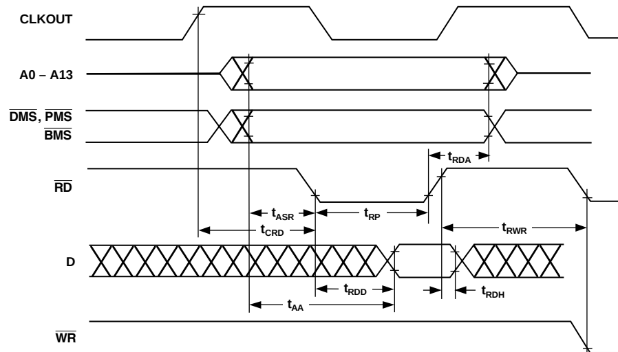
Figure 32. Memory Read
