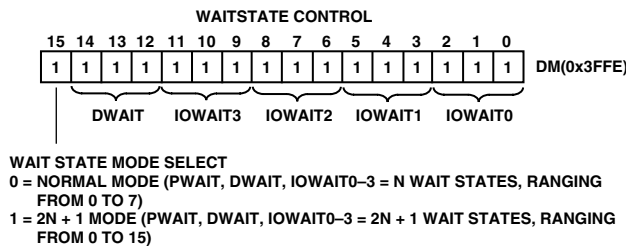
Figure 6. Wait State Control Register
