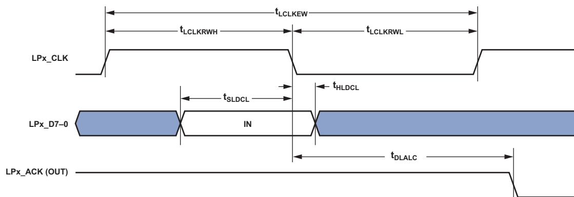
Figure 10. LPs—Receive
