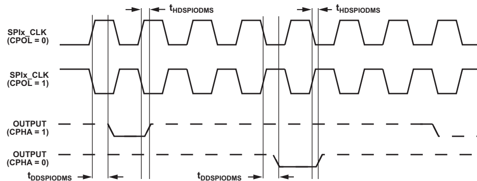
Figure 22. ODM Slave Mode
