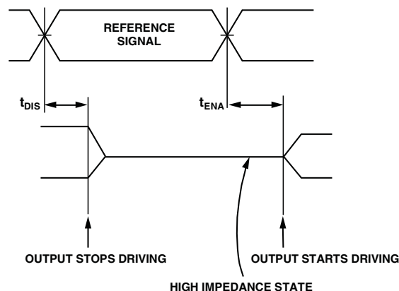
Figure 46. Output Enable/Disable
