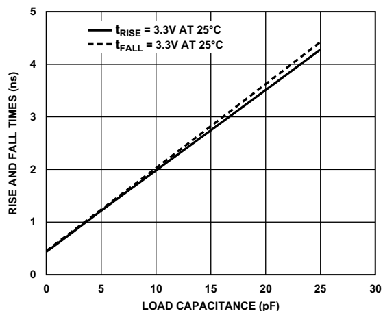
Figure 49. Driver Type A Typical Rise and Fall Times (10% to 90%) vs. Load Capacitance for All GPIO/DAI Pins Operating at Less Than 62.5 MHz ( V_{DD\_EXT} = 3.3\text{ V} )
