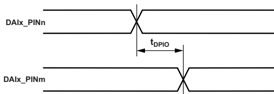
Figure 29. DAI Pin to DAI Pin Direct Routing
