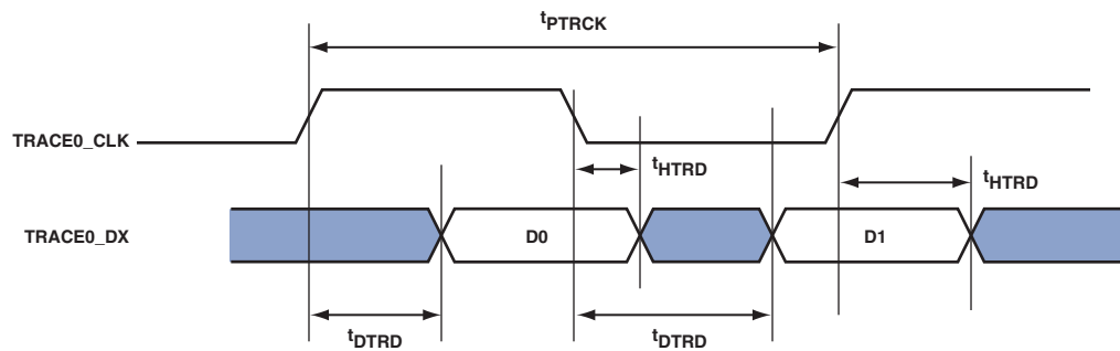
Figure 37. Trace Timing
