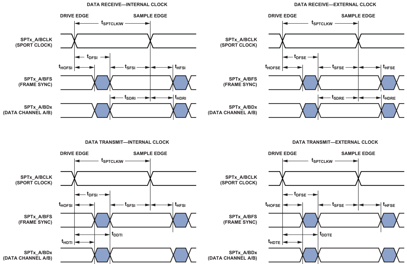
Figure 12. SPORTs
