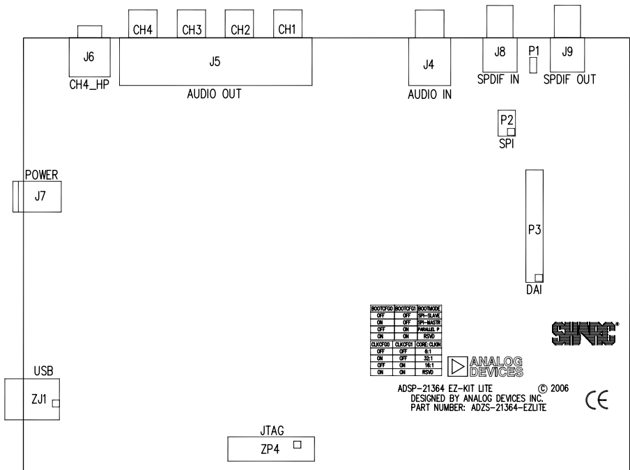
Figure 2-7. Connector Locations
