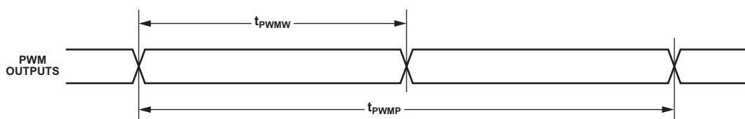
Figure 26. PWM Timing
