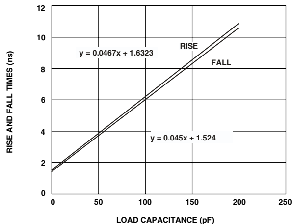
Figure 31. Typical Output Rise Time (20%–80%, V_{DDEXT} = \text{Max} )
