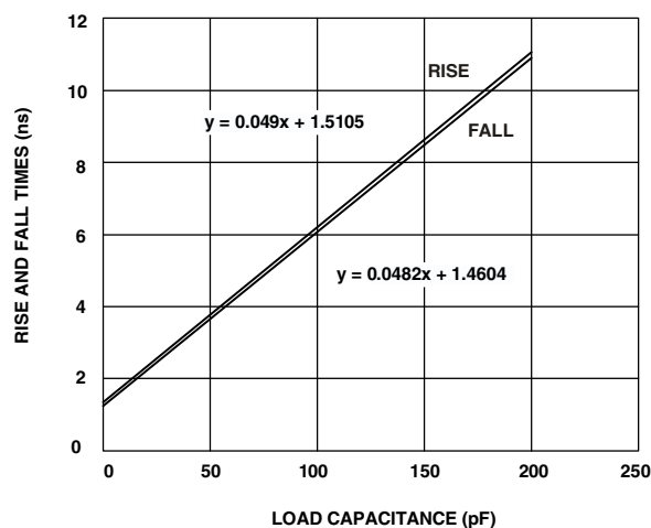
Figure 32. Typical Output Rise/Fall Time (20% to 80%, VDDEXT = Min)
