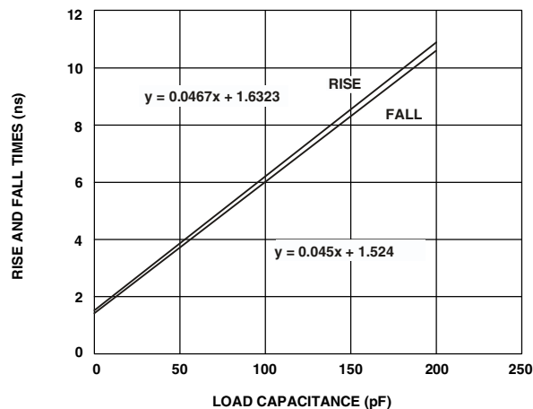
Figure 31. Typical Output Rise Time (20% to 80%, V DDEXT = Max)
