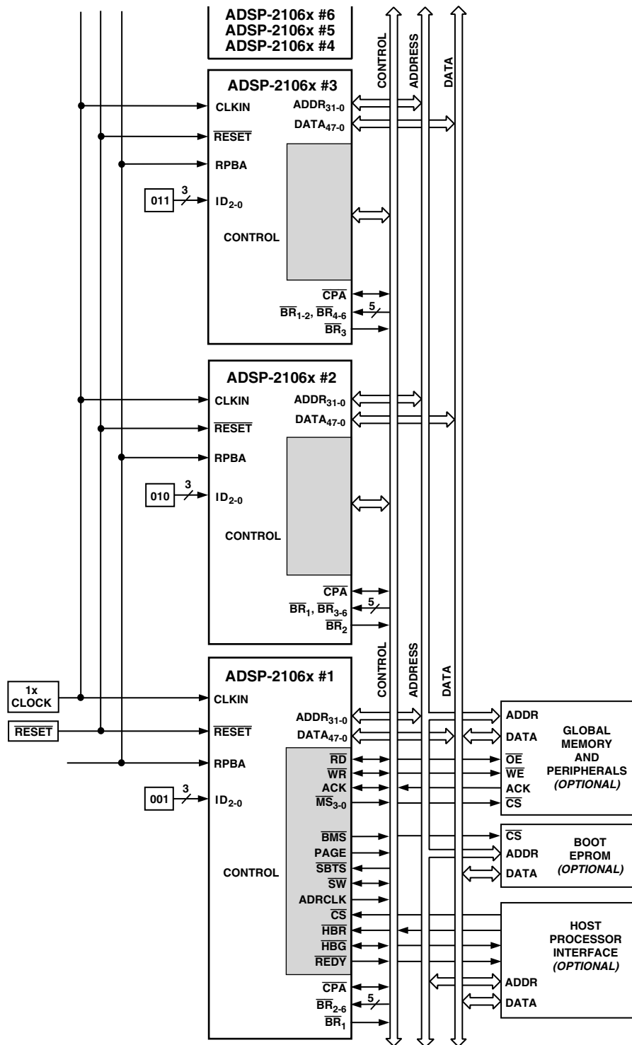
Figure 3. Multiprocessing System
