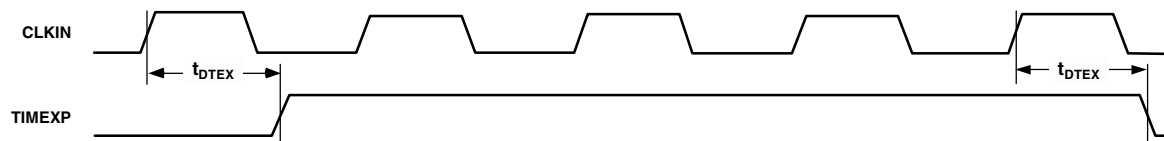
Figure 12. Timer
