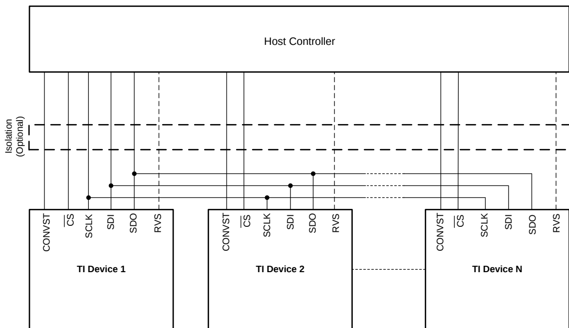
Figure 90. Star-Topology Connection
