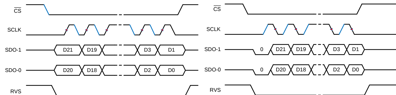
Figure 60. SPI-00-D Protocol
