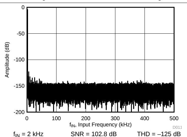
Figure 21. Typical FFT
