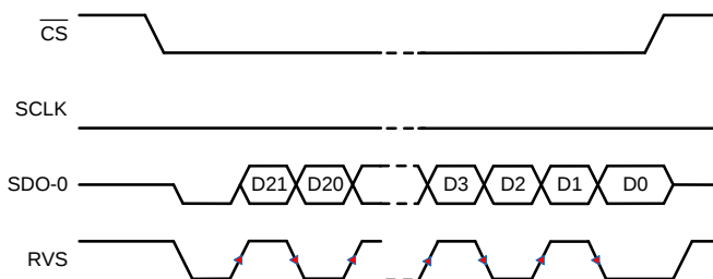
Figure 76. SRC-INT-SD: SRC, INTCLK, Single SDO, DDR
