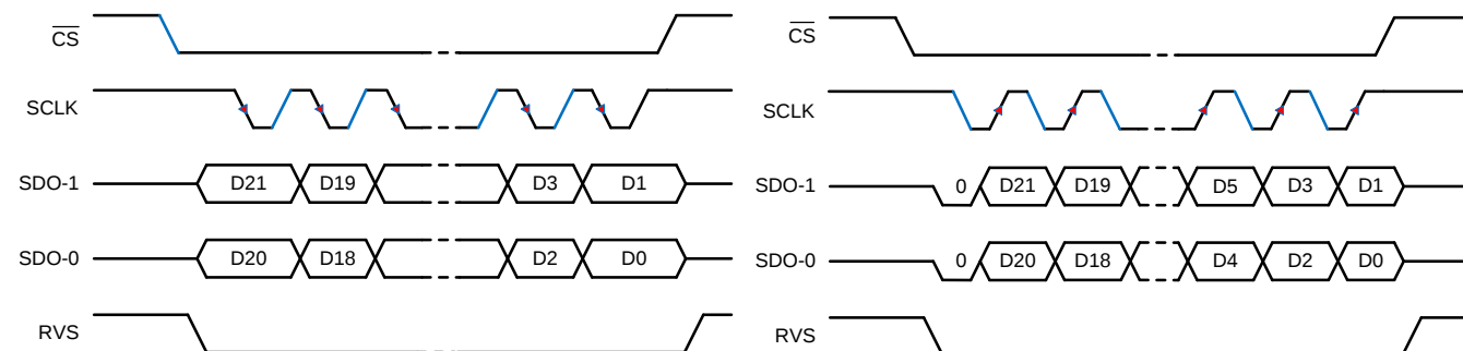
Figure 62. SPI-10-D Protocol
