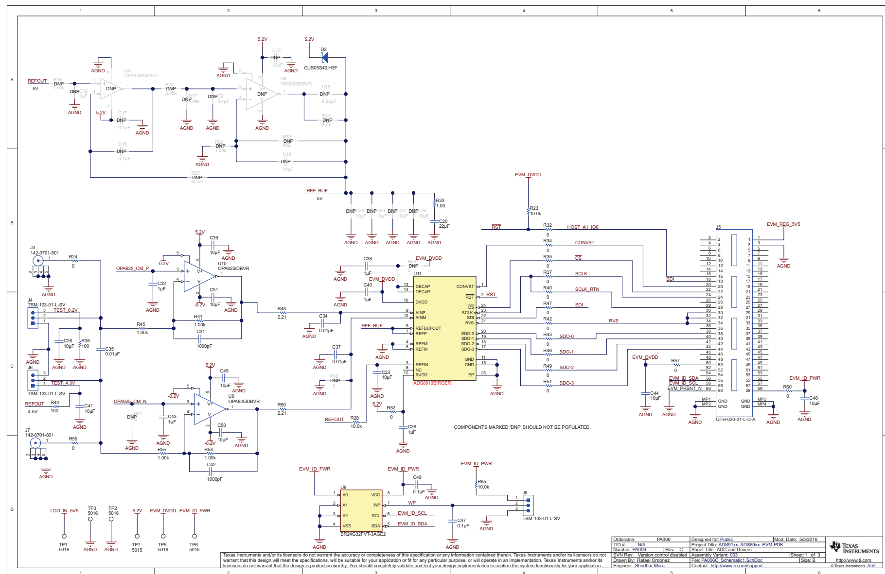
Figure 20. Schematic Diagram (Page 1) of the ADS8910BEVM PCB
