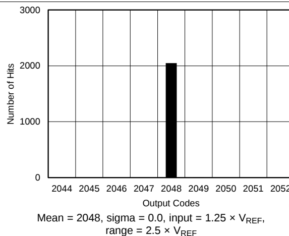
Figure 9. DC Histogram for Mid-Scale Inputs ( 2.5 \times V_{REF} )
