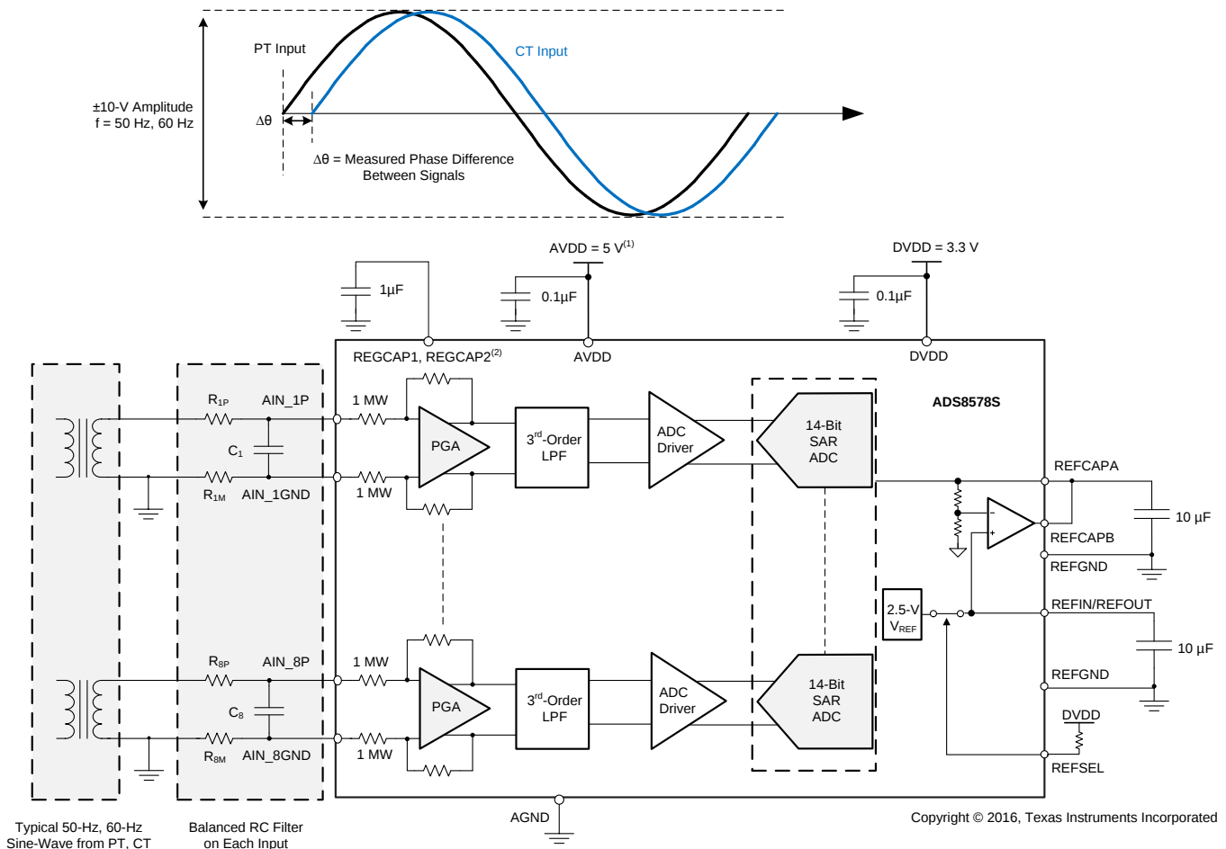
Figure 84. 8-Channel DAQ for Power Automation Using the ADS8578S
