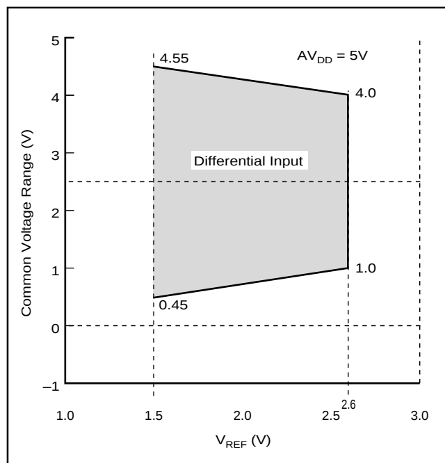
FIGURE 4. Differential Input: Common-Mode Voltage Range vs V_{REF} .
