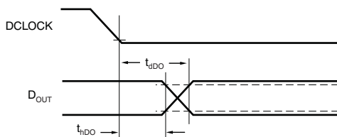
Voltage Waveforms for D_{OUT} Delay Times, t_{dDO}
