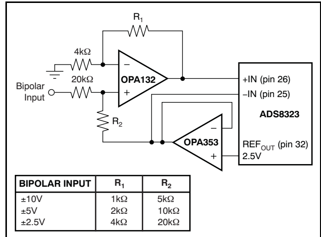
Figure 21. Level Shift Circuit for Bipolar Input Ranges
