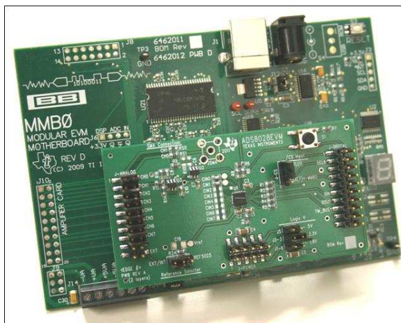
Figure 1. ADS8028EVM-PDK
