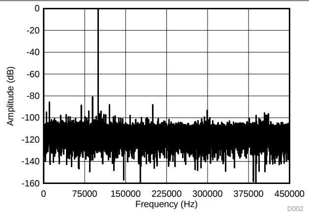
Figure 31. Test Results for the ADS7886 and OPA365 for a 100-kHz Input
