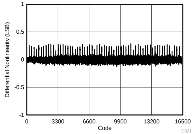
Figure 22. Typical DNL
