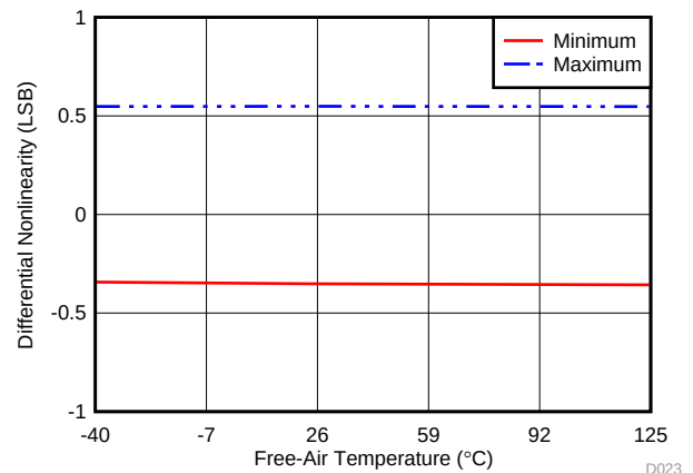
Figure 22. Typical DNL
