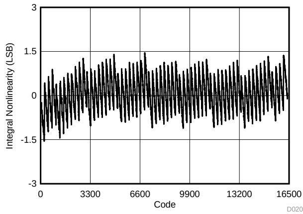
Figure 21. Typical INL
