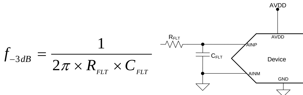
Figure 40. Antialiasing Filter
