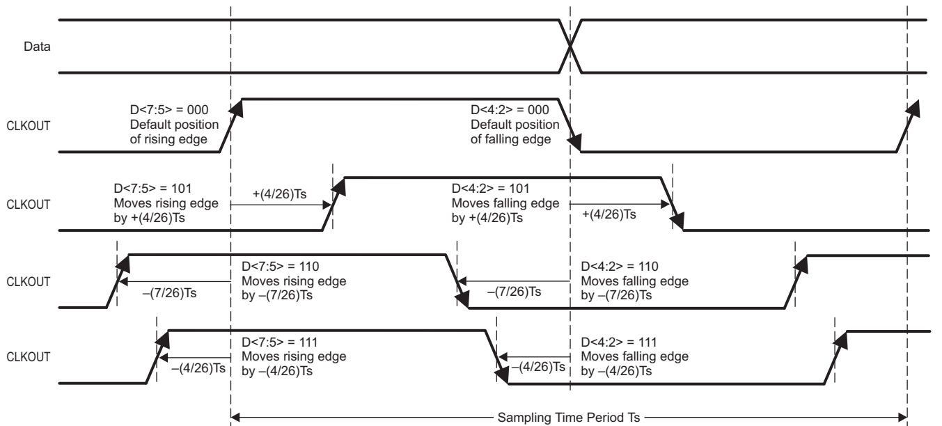
Figure 12. LVDS Interface Output Clock Edge Movement (Serial Register 0x44)
