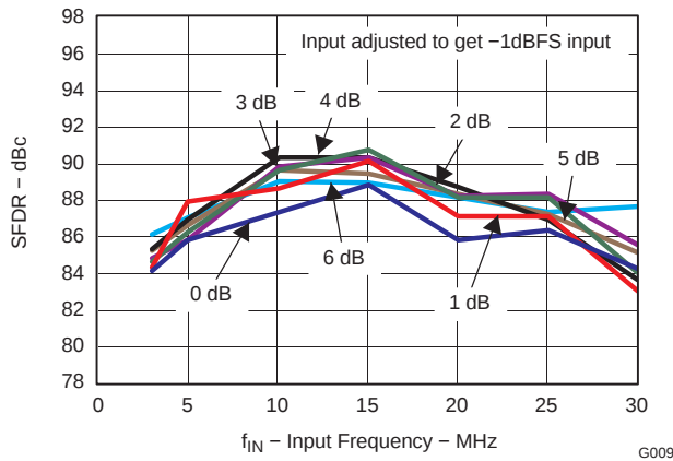
Figure 12. SFDR Across Fine Gain
