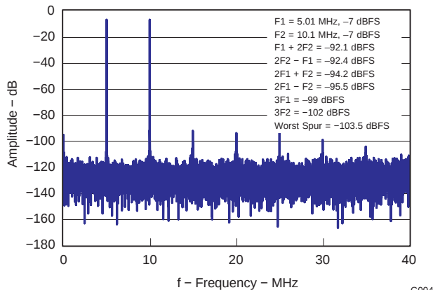
Figure 9. Intermodulation Distortion
