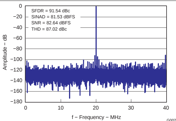
Figure 7. FFT for 20 MHz, -1-dBFS Input Signal
