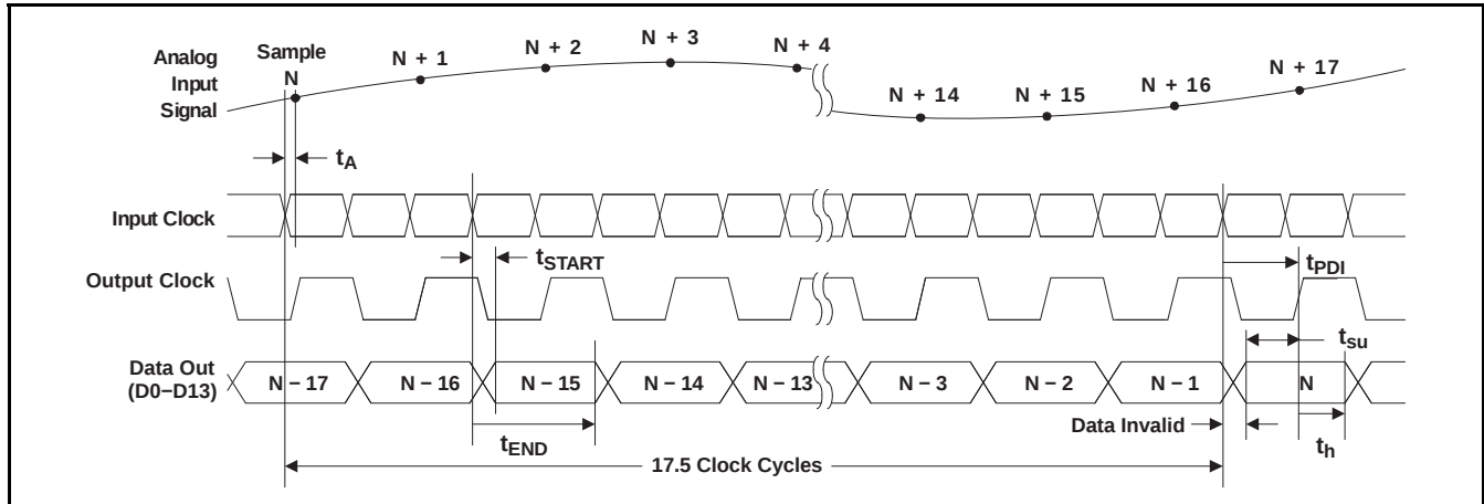
Figure 1. Timing Diagram
