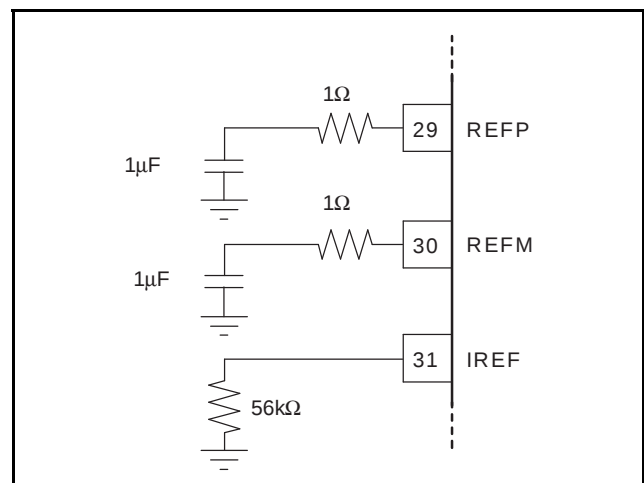
Figure 44. REFP, REFM, and IREF Connections for Optimum Performance
