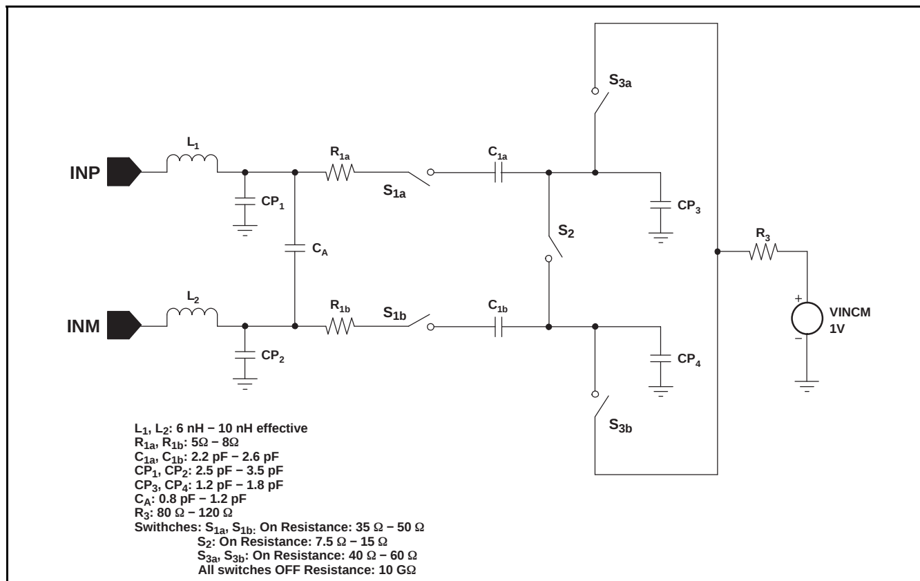
Figure 39. Analog Input Stage
