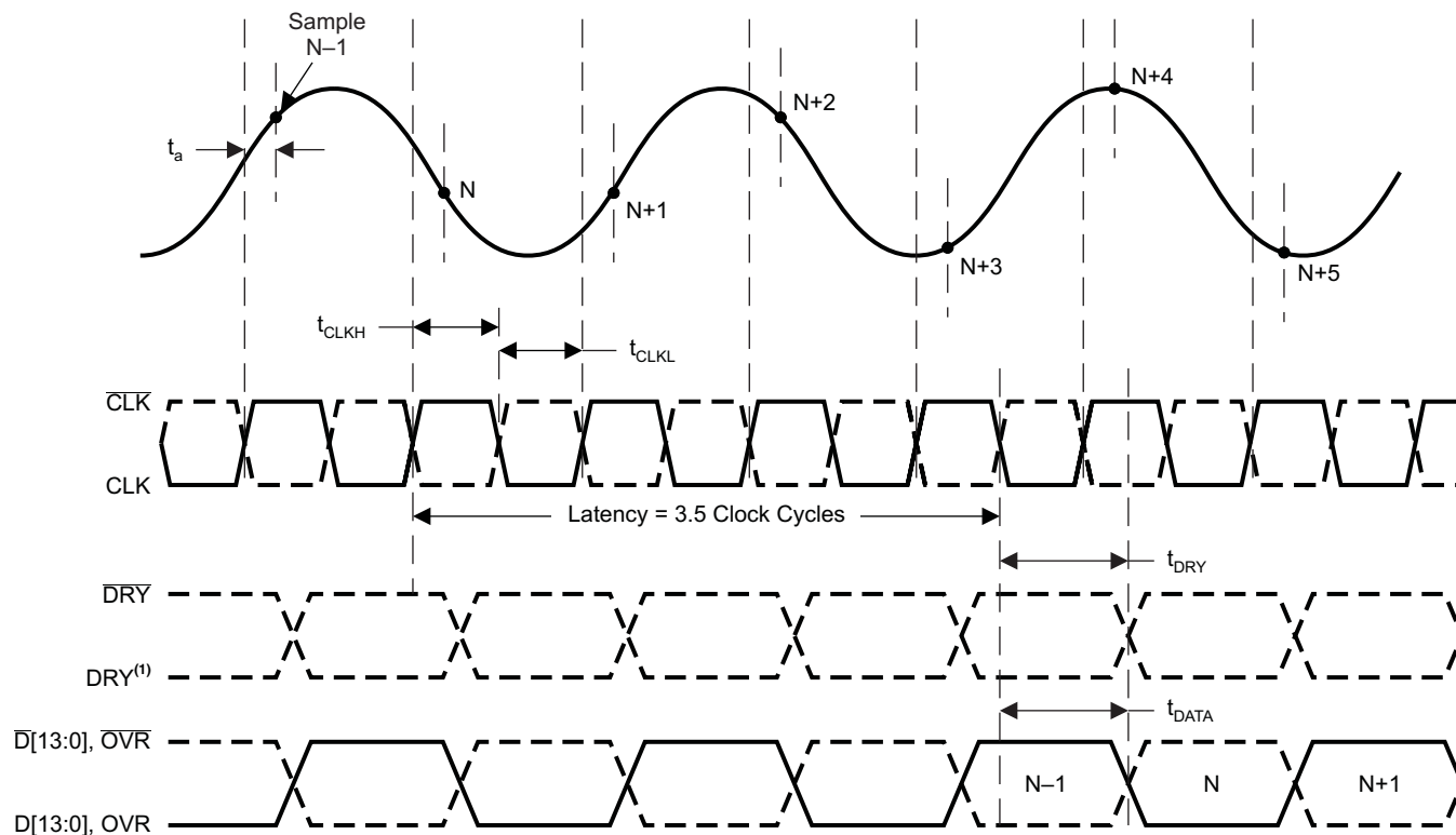
Figure 1. Timing Diagram
