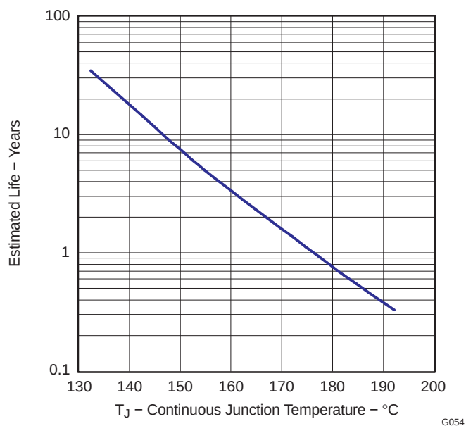
Figure 69. Operating Life Derating Chart, Wirebond Voiding Fail Mode
