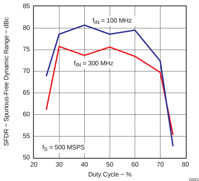
Figure 64. ADS5463 SFDR vs Clock Duty Cycle
