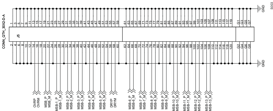
Figure 12. EVM Schematics
