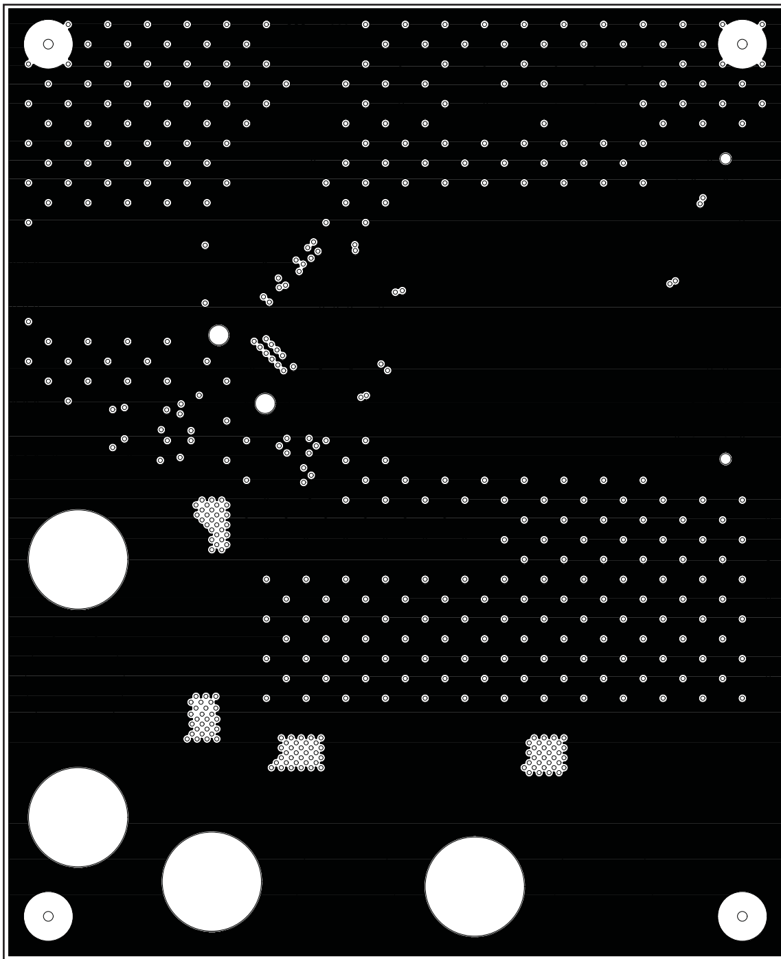
Figure 5. Ground Plane 1
