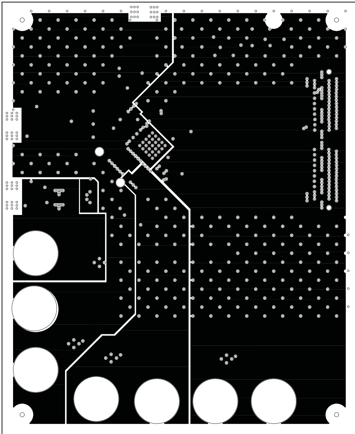
Figure 7. Power Plane 2
