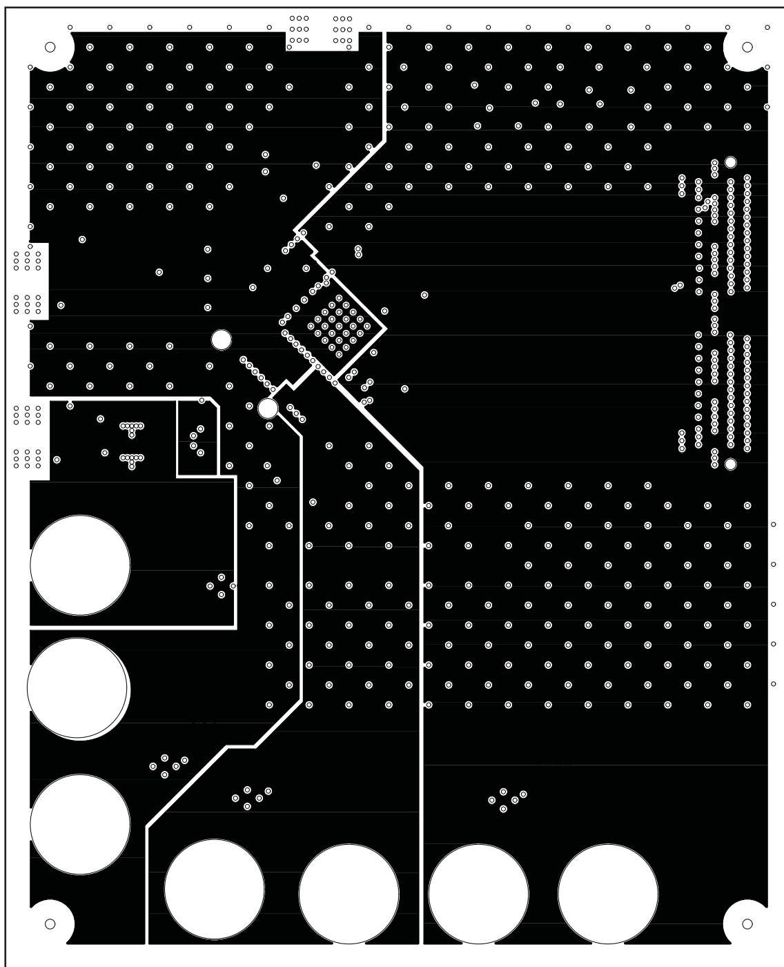
Figure 6. Power Plane 1
