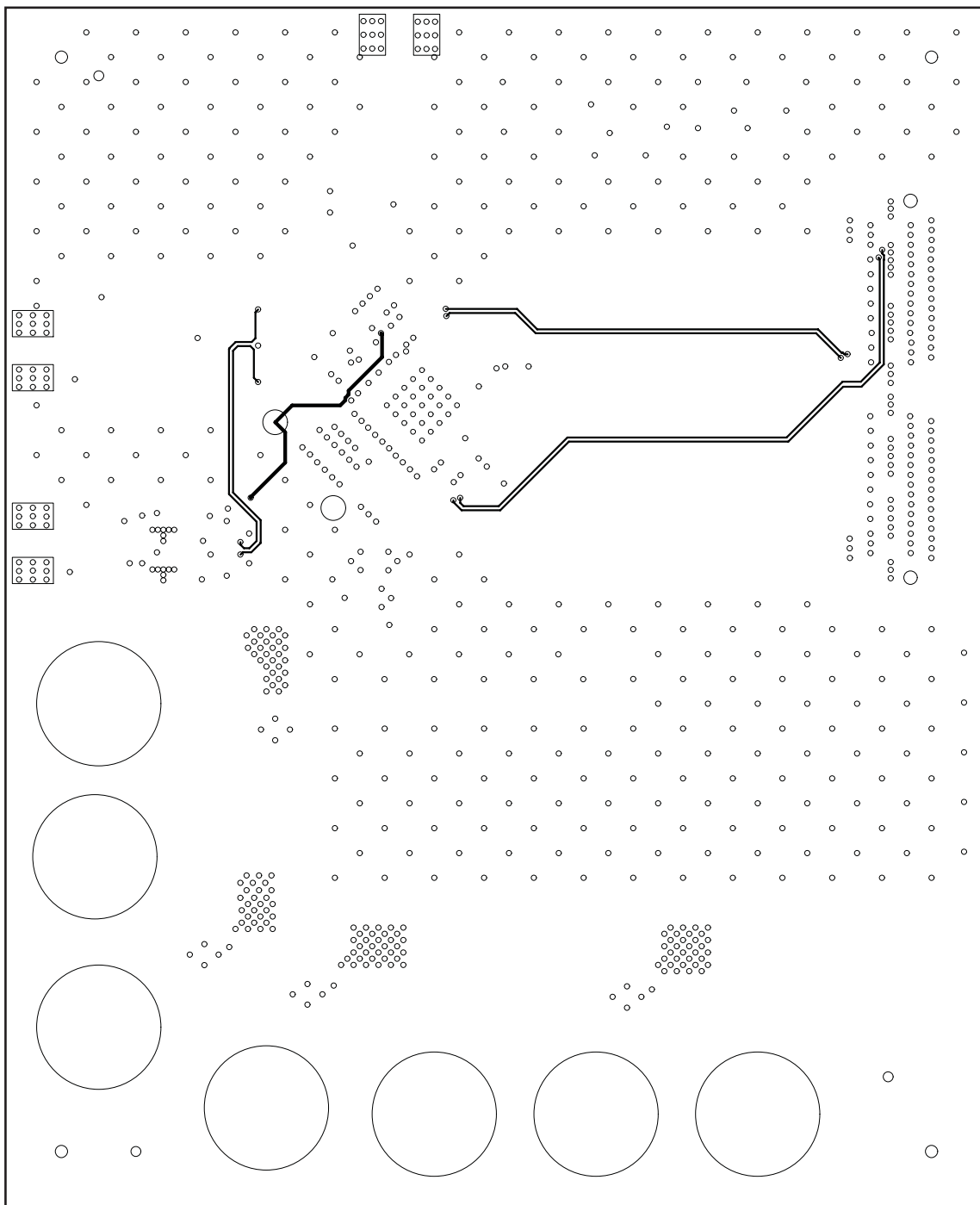
Figure 9. Bottom Side
