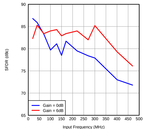
Figure 11. SFDR vs Input Frequency
