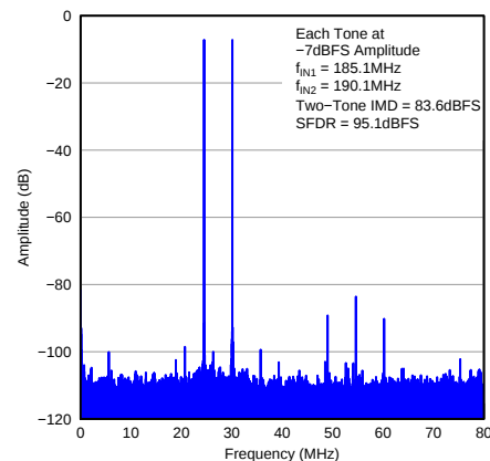
Figure 9. FFT for Two-tone Input Signal
