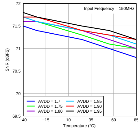
Figure 63. SNR vs Temperature and AVDD Supply
