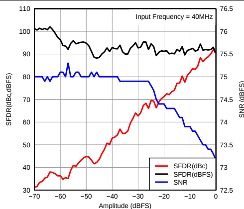
Figure 37. Performance vs Input Amplitude
