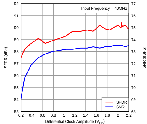
Figure 65. Performance vs Input Clock Amplitude
