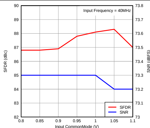
Figure 39. Performance vs Input Common-Mode Voltage
