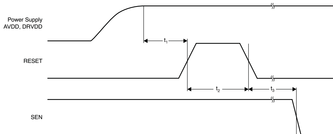
Figure 152. Serial Readout Timing Diagram
