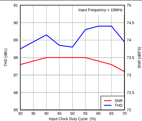
Figure 67. Performance Across Input Clock Duty Cycle
