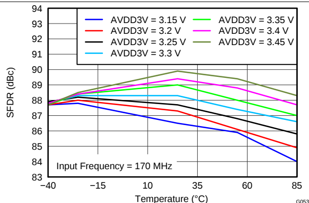
Figure 51. SFDR vs AVDD Supply and Temperature (170 MHz)
