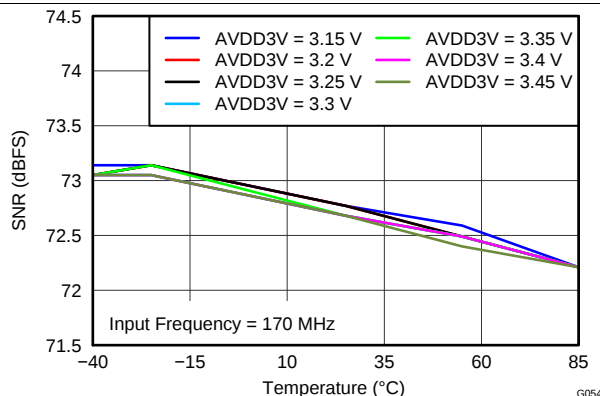
Figure 52. SNR vs AVDD Supply and Temperature (170 MHz)
