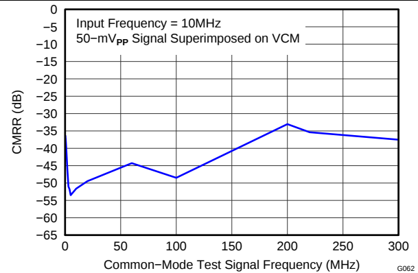
Figure 62. CMRR vs Test Signal Frequency
