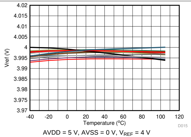
Figure 16. Internal V_{REF} vs Temperature
