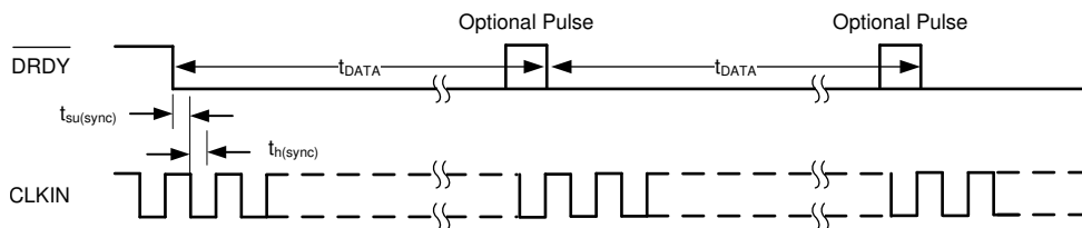
Figure 4. \overline{DRDY} Synchronization Timing for Synchronous Slave Mode (CLKSRC = 0)
