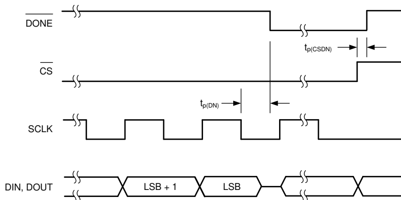
Figure 6. \overline{DONE} Signal Timing
