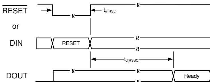
Figure 7. \overline{RESET} Pin and Command Timing
