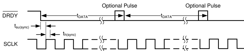
Figure 5. \overline{DRDY} Synchronization Timing for Synchronous Slave Mode (CLKSRC = 1)
