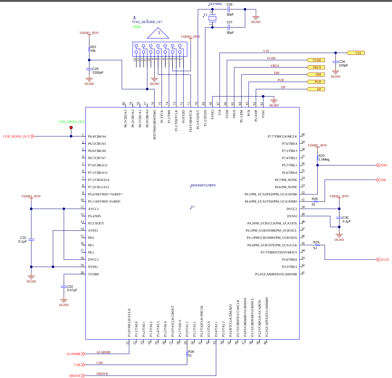
Figure 13: ADS1293EVM Schematic
