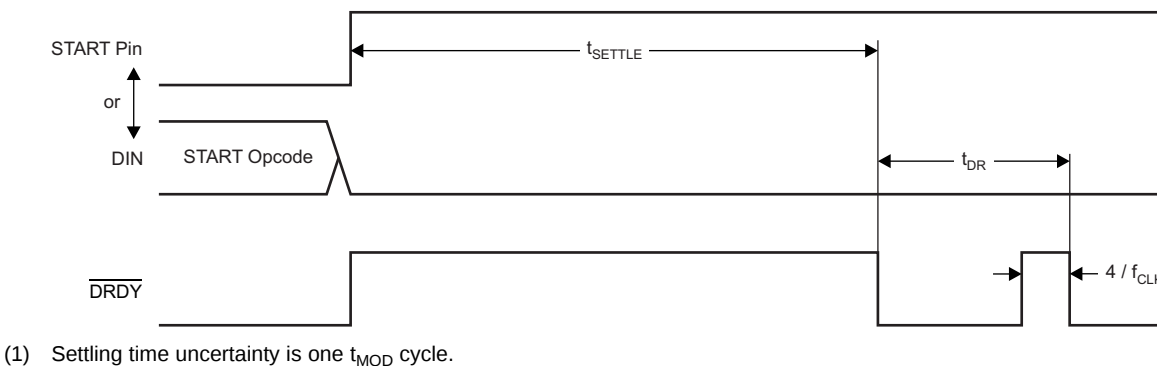
Figure 48. Settling Time
