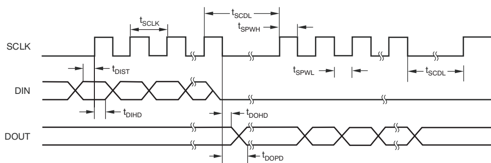
Figure 1. Timing Diagram
