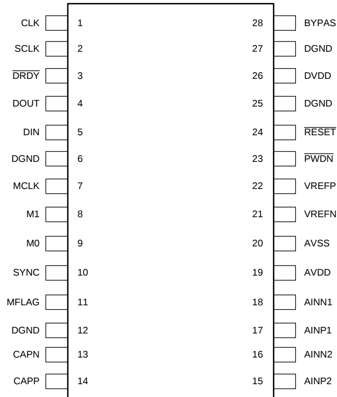
Pin Functions
