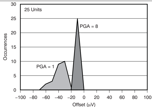
Figure 20. Offset Histogram
