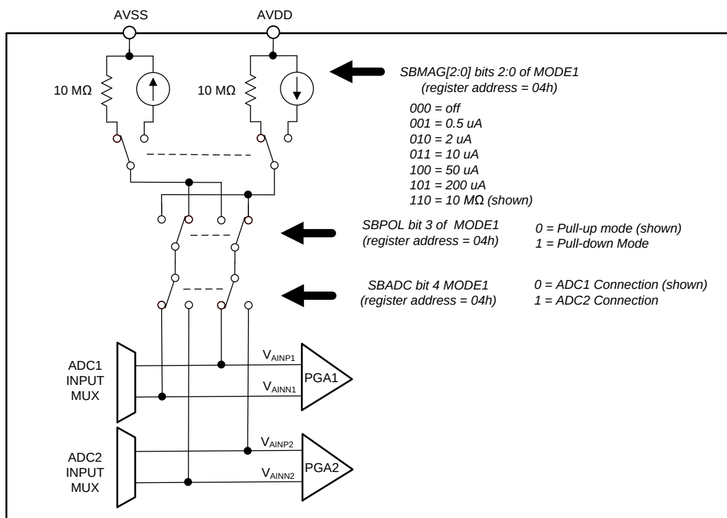
Figure 68. Sensor Bias Block Diagram
