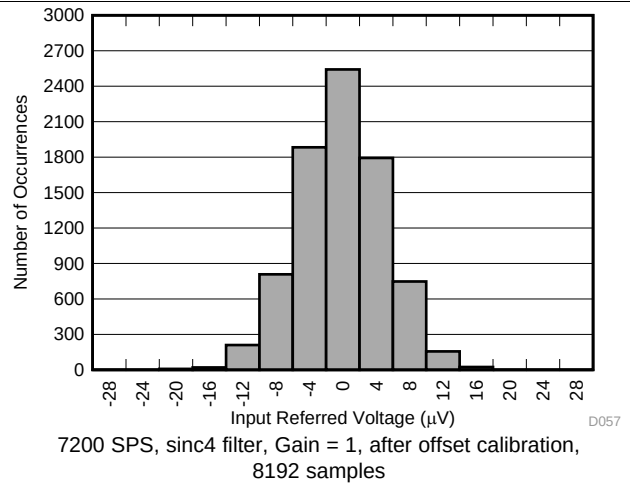
Figure 17. ADC1 Output Reading Distribution
