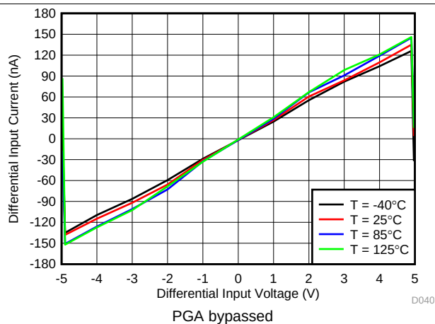
Figure 25. ADC1 Differential Input Current
