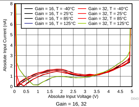
Figure 28. ADC1 Absolute Input Current
