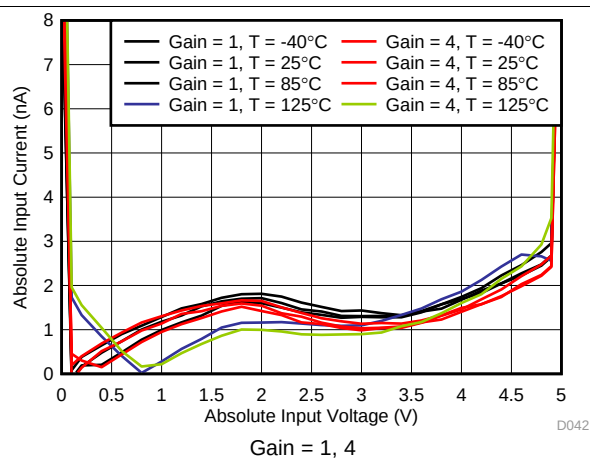
Figure 27. ADC1 Absolute Input Current
