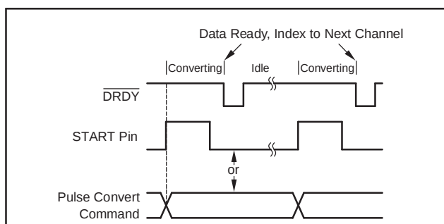
Figure 55. Pulse Conversion, Auto-Scan Mode
