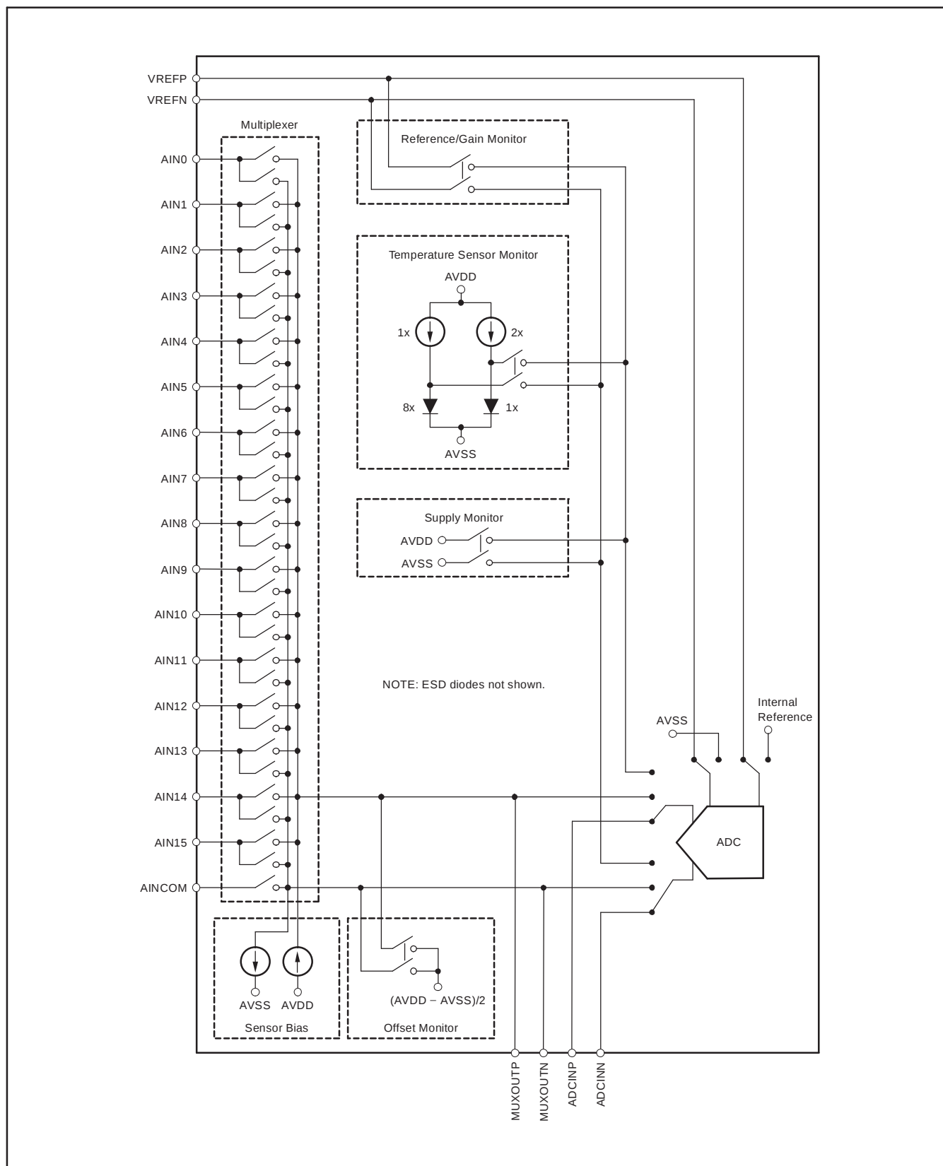
Figure 36. Input Multiplexer
