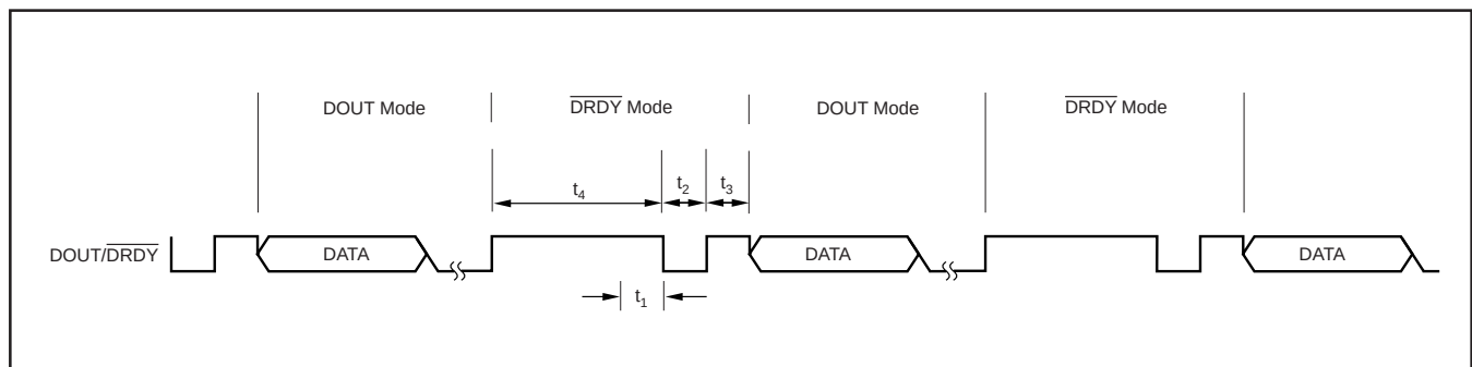
FIGURE 11. DOUT/DRDY Partitioning.
