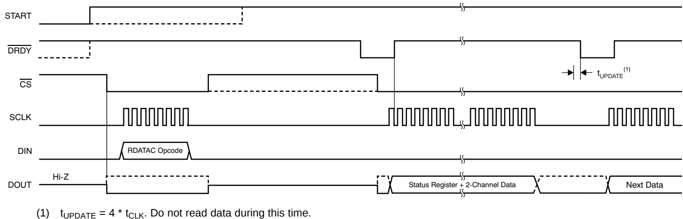
Figure 38. RDATAC Usage
