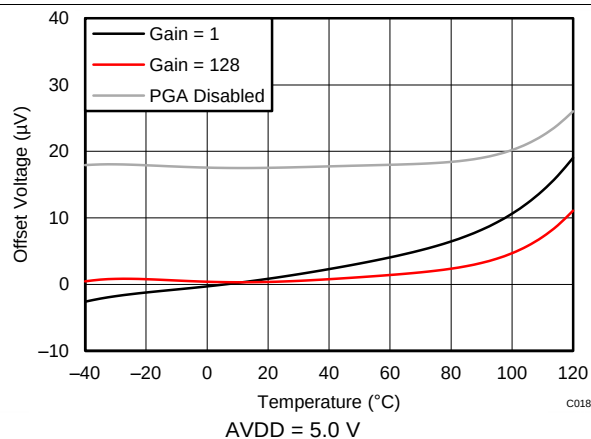
Figure 4. Input-Referred Offset Voltage vs Temperature
