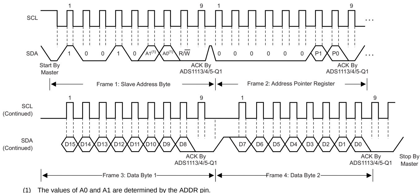
Figure 31. Timing Diagram for Writing to ADS111x-Q1
