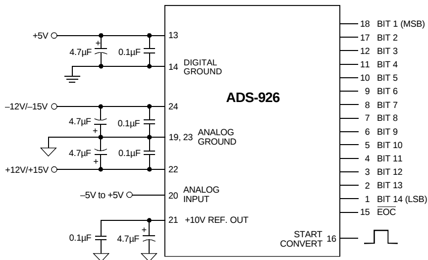
Figure 3. Typical ADS-926 Connection Diagram
