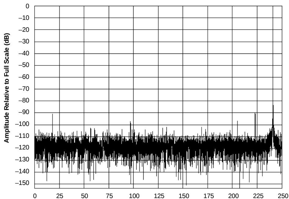
Figure 6. ADS-926 FFT Analysis
